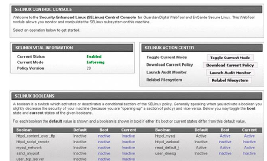
Figure 4. Selinux control
